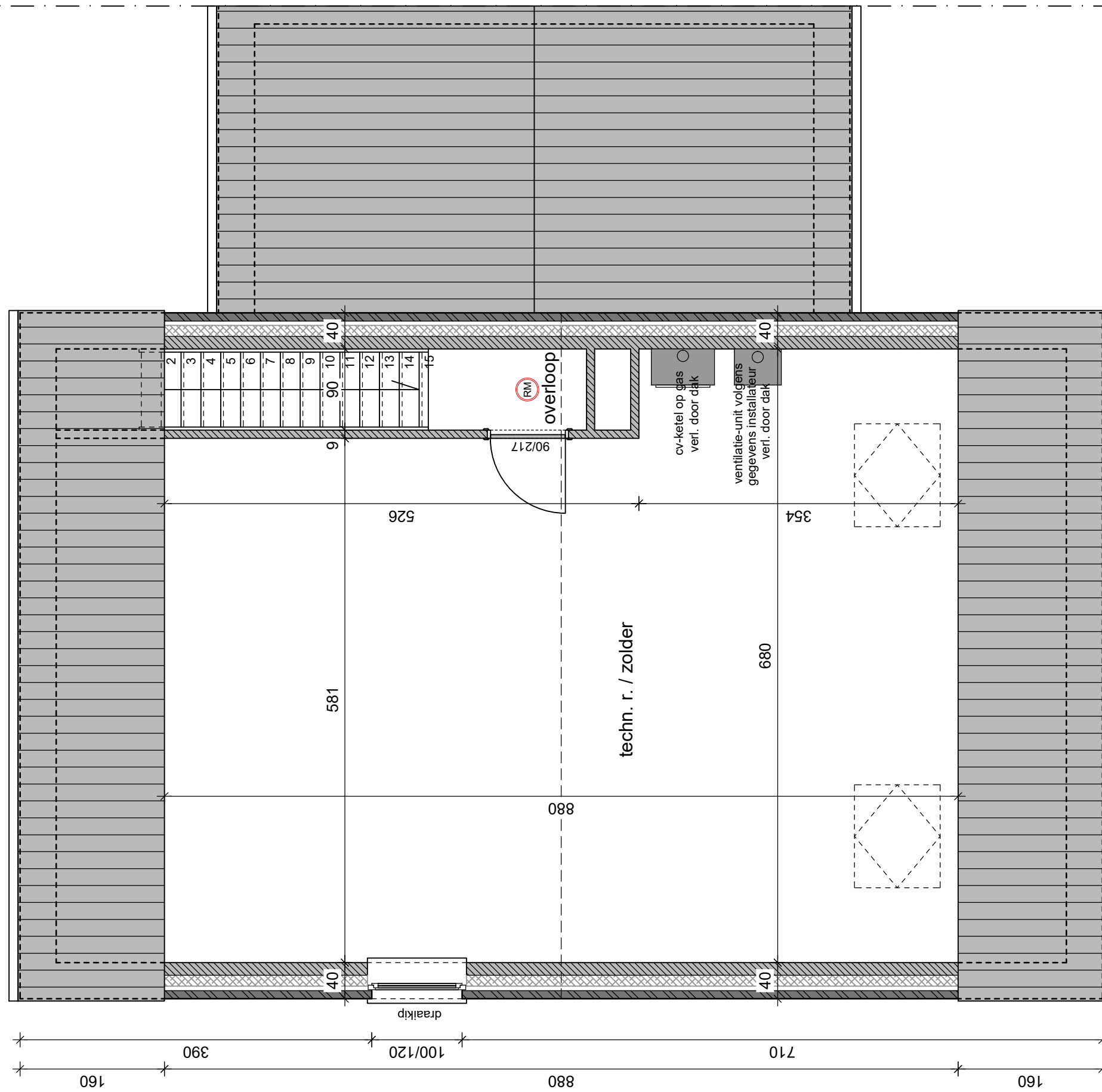
plan zolder
