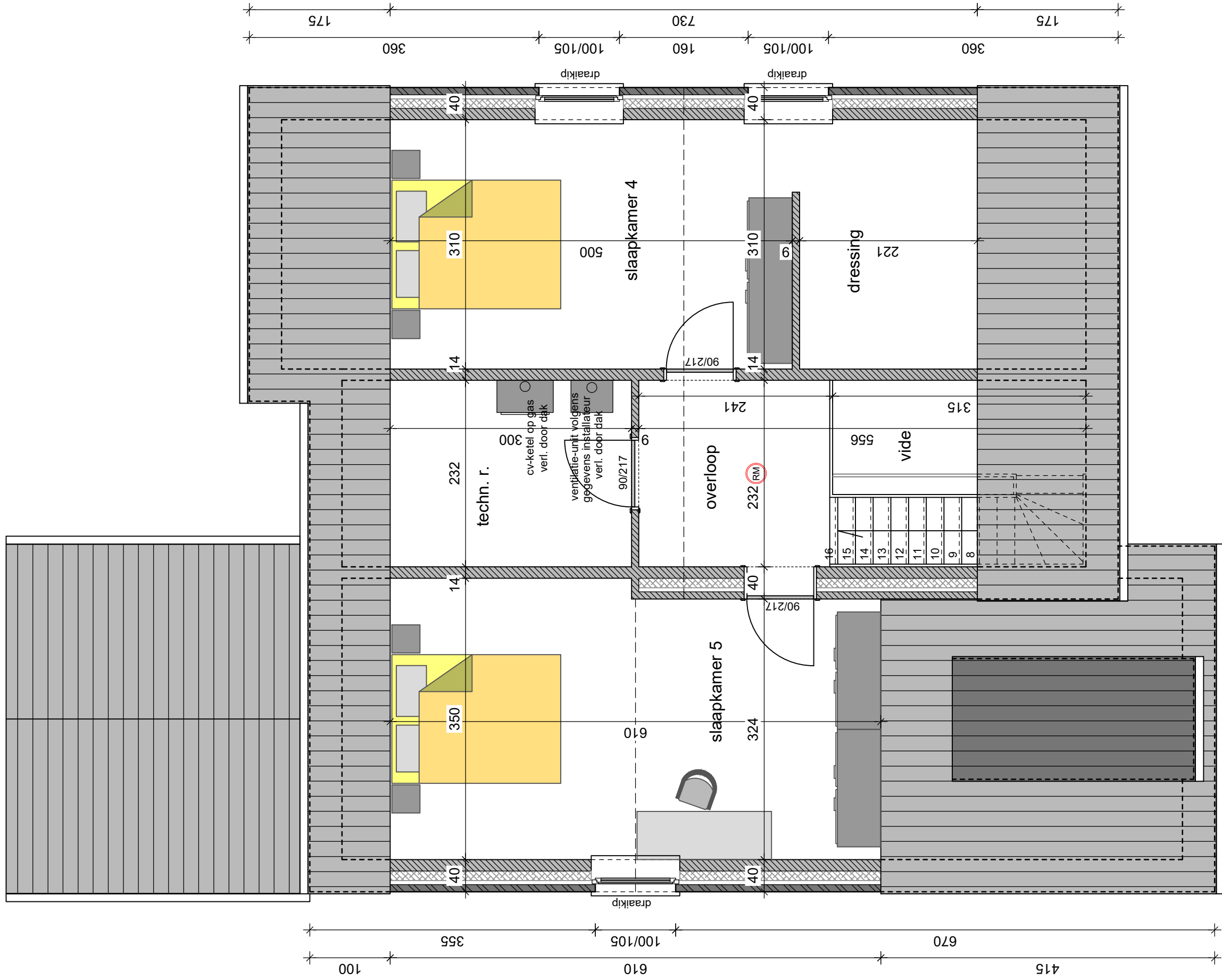
plan zolder
