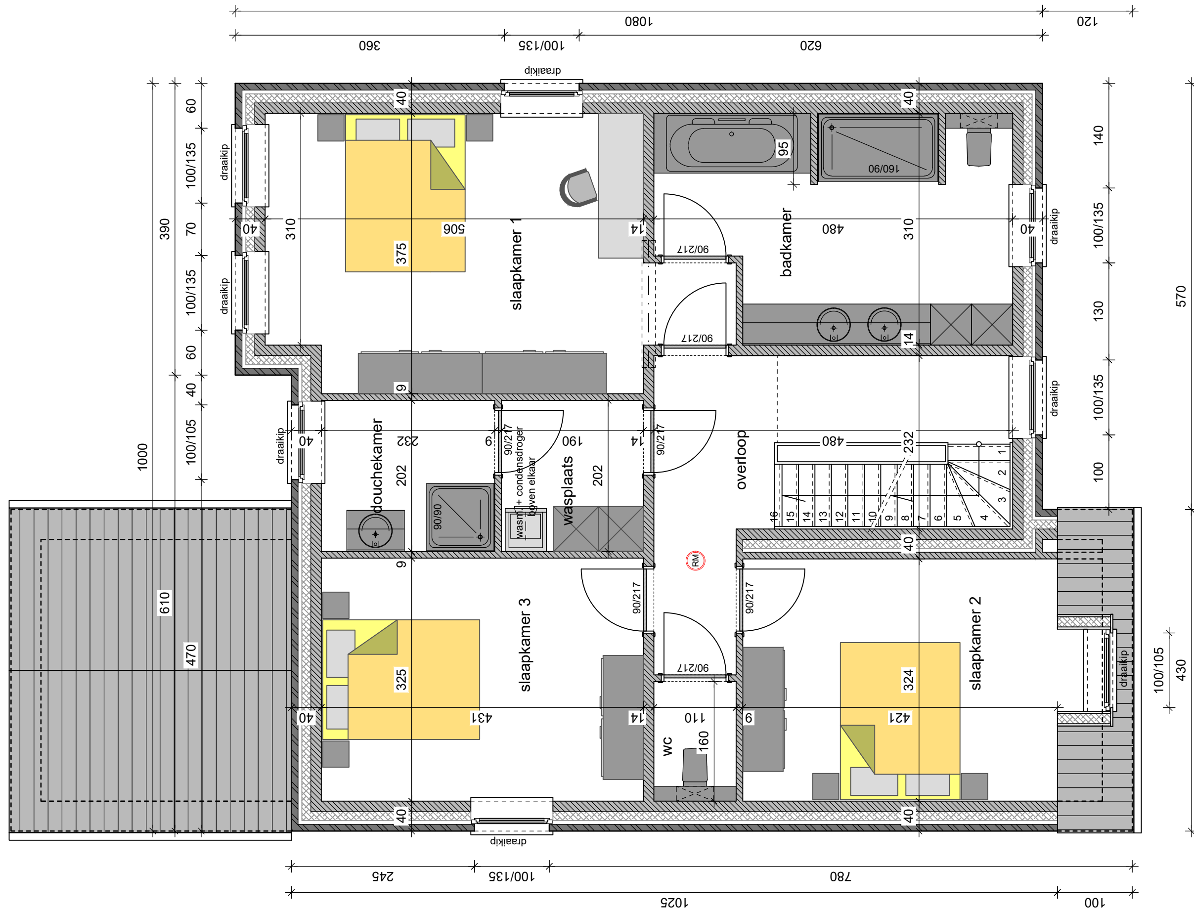
plan verdieping
